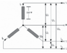
Star connection
