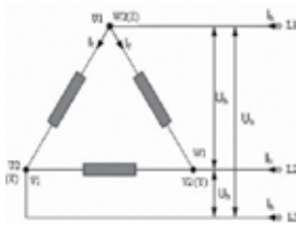
Delta connection
