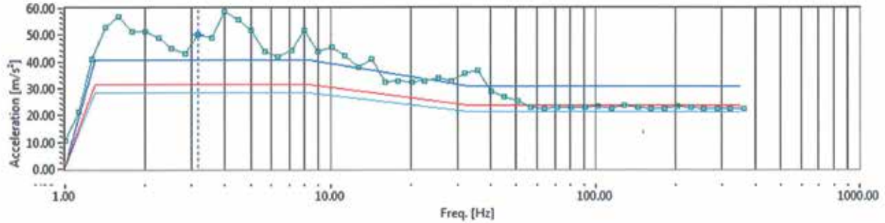
Figure 12 – Seismic Test Result – 800mm Tubeaxial Fan – X-Direction – Response Spectra
